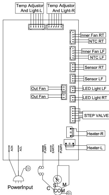
Electrocircuit Line Diagram
