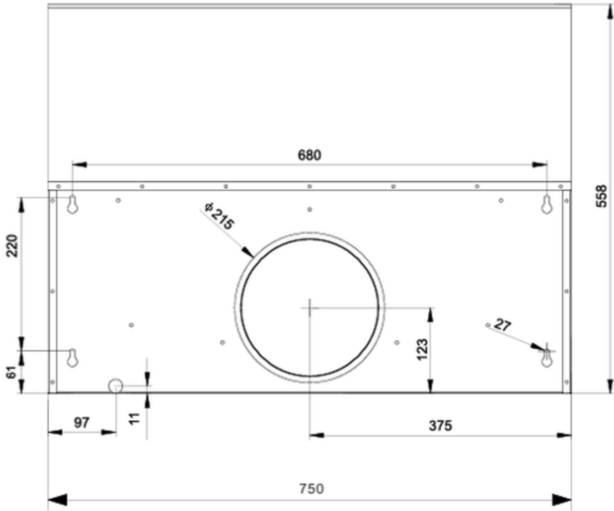
Top View (mm)
