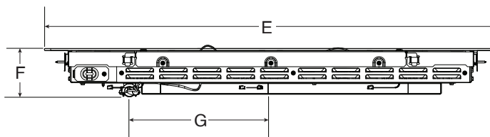
VISTA FRONTAL
