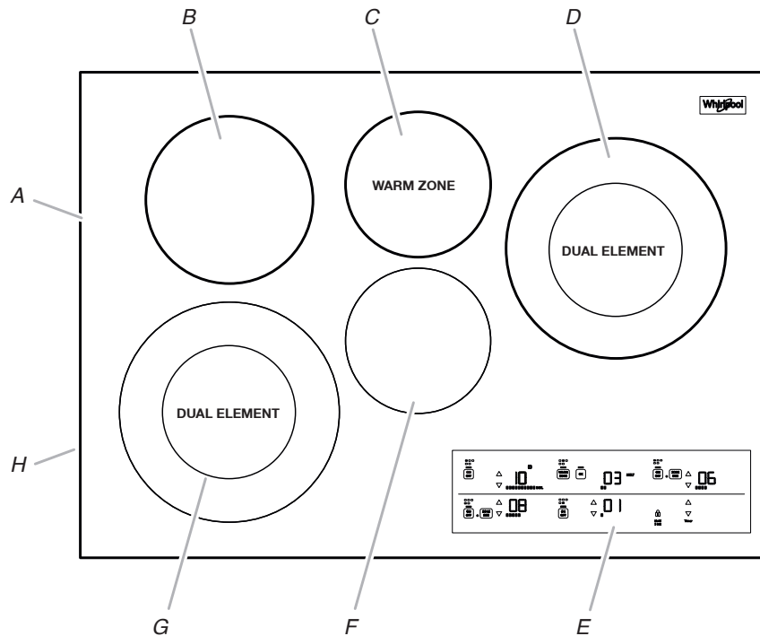
30" (76.2 cm) Model WCE97US0K Touch-Activated Electronic Control Model shown
