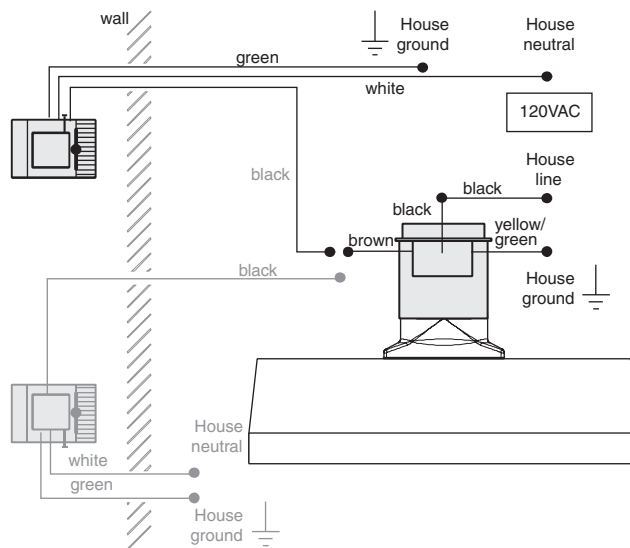
10" (25.4 cm) Makeup air installation
