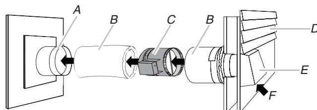
A. Wall register B. Ducts C. 6" (15.2 cm) motorized damper
