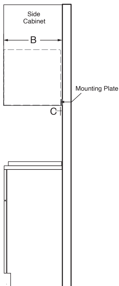
SIDE VIEW
