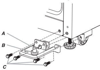
A. Bottom Hinge B. Washer C. 1/16" Hex-Head Hinge Screws
