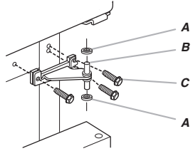
A. Washer B. Center Hinge C. 1/16" Hex-Head Hinge Screws
